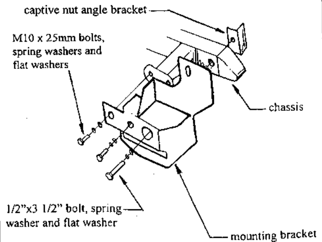
Diagram 6 - Mounting bracket
