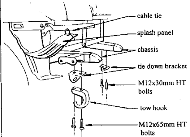
Diagram 4 - Pre-assembly
