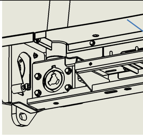
Pan Cover
